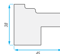
MOULDING PROFILE
