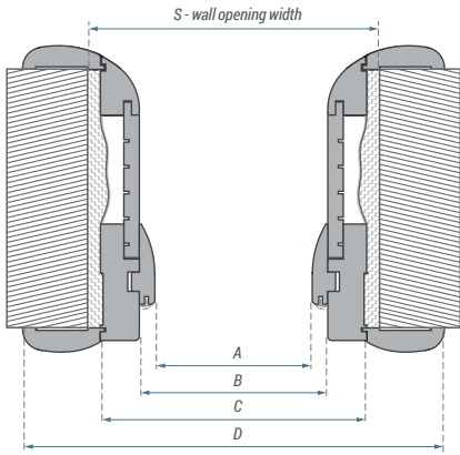
Dimensions of New Arcus door frame [mm]:
