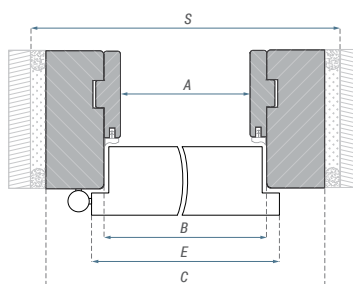
Dimensions of FIRE wooden fixed and adjustable door frame [mm]:
