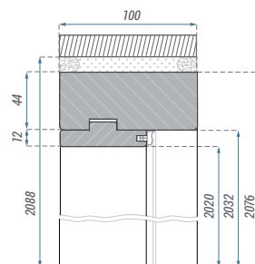
42 DB MDF FIXED ▼
