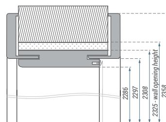
▼ Dimensions of door frame for Natura HB PN23 door.
