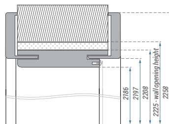
▲ ADJUSTABLE DOOR FRAME NON-REBATED
