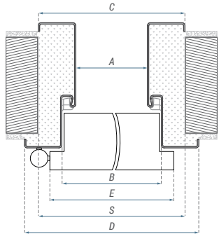
Dimensions of FIRE steel fixed door frame [mm]:
