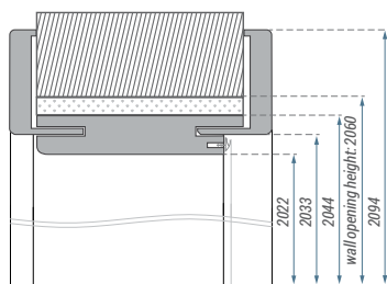
▼ Dimensions of door frame for Natura HK PN22 door.
