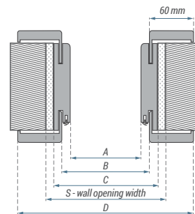
▼ Dimensions of door frame for Natura HK PN23 door.
