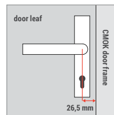
3. Handle and rosette dimensions. Door handle cannot extend beyond the spindle.
