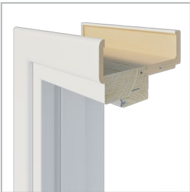
COMPLETE DOOR FRAME WITH ADJUSTMENT BAND AND OVERLAY MOULDING
