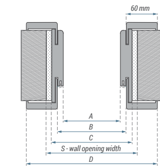
▼ Dimensions of door frame for Natura HB PN23 door.
