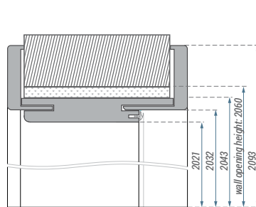
▼ Dimensions of door frame for Natura HB PN22 door.
