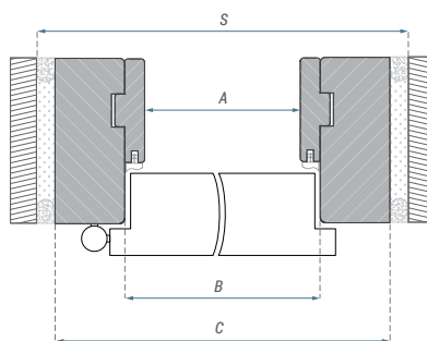
Dimensions of 42dB MDF fixed door frame [mm]:
