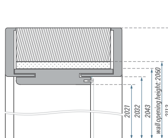
▼ ADJUSTABLE DOOR FRAME NON-REBATED 80
