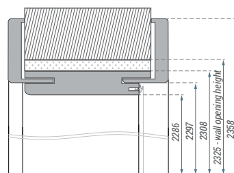
▼ Dimensions of door frame for Natura HK PN23 door.
