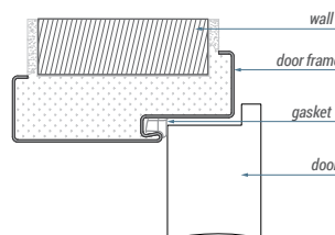
GUARD STEEL FIXED ▼
